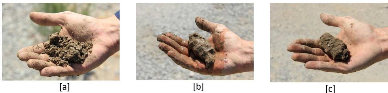
Figure 64. Photo. Squeeze test for assessing moisture content. ([a] too dry, [b] too wet, and [c] acceptable)
