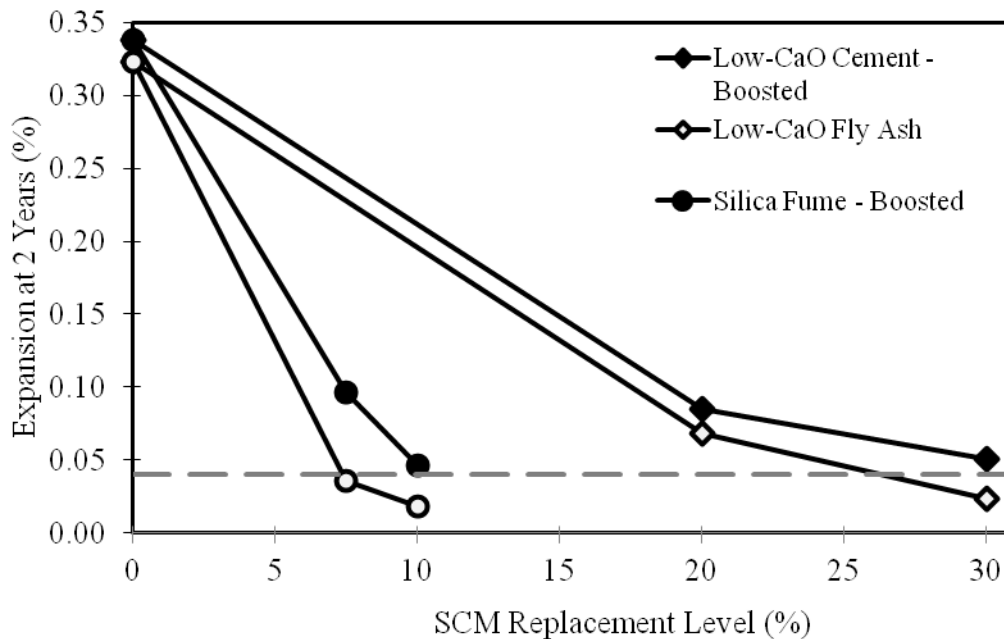
Figure 5.18. Effect of Cement Alkalies on Expansion of Concrete Containing Fly Ash or Silica Fume (Fournier et al. 2004)
