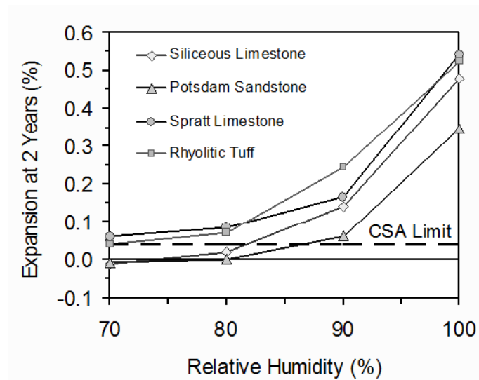
Figure 2.16. Effect of Relative Humidity on Expansion of Concrete Prisms (Pedneault 1996)
