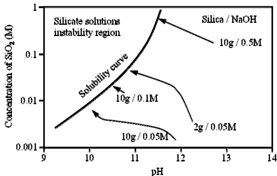
Figure 2.4. Equilibrium Solubility Curve ( \text{SiO}_2 -pH) and Change in Composition for Different Solutions of \text{SiO}_2 -NaOH (from Dent Glasser and Kataoka 1981b)
