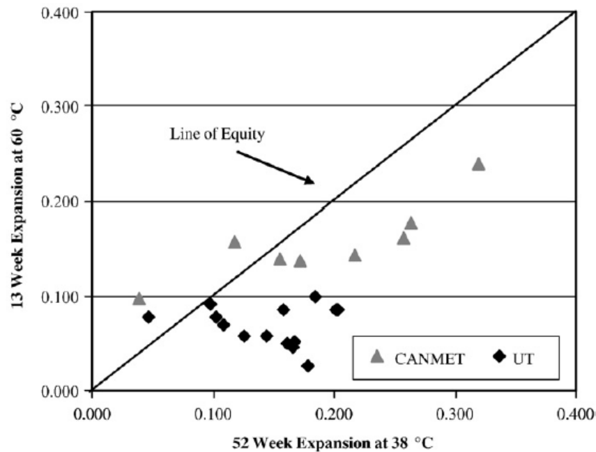
Figure 4.4. Relationship between Expansion after One Year Using the Standard CPT (38°C) and the Expansion after 13 Weeks Using the Accelerated CPT (60°C) (Ideker et al. 2010)
