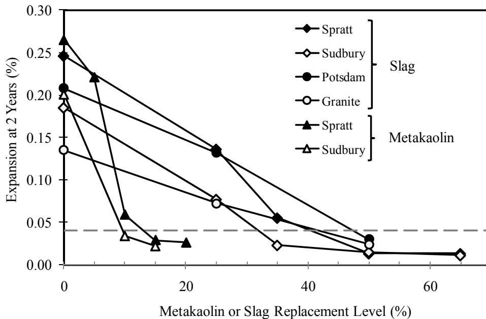
Figure 5.19. Effect of Aggregate Type on the Amount of Metakaolin or Slag Required to Control ASR Expansion (Thomas and Innis 1996; Ramlochan et al. 2000)
