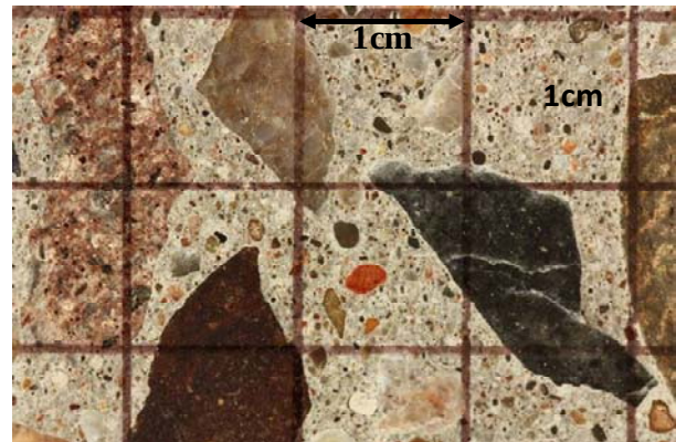
Figure 7.13. Examination of the polished concrete section under the stereomicroscope for the determination of the Damage Rating Index . Petrographic features of deterioration (Table 7.8; Figure 7.7) are counted in a one cm x one cm grid system drawn at the surface of the polished concrete section.
