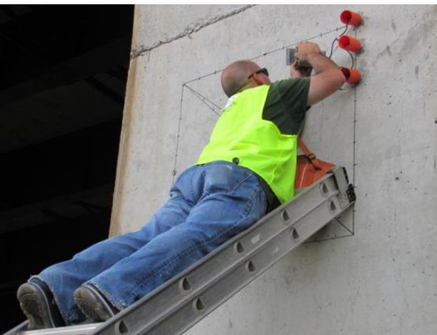
Figure 7.11. In-situ measurements of humidity in concrete. A. Wooden-stick method. B-C. Portable humidity probes. D. Automatic in-situ monitoring of temperature, humidity and expansion (vibrating wire) in a bridge deck affected by ASR (Siemes and Gulikers 2000).
