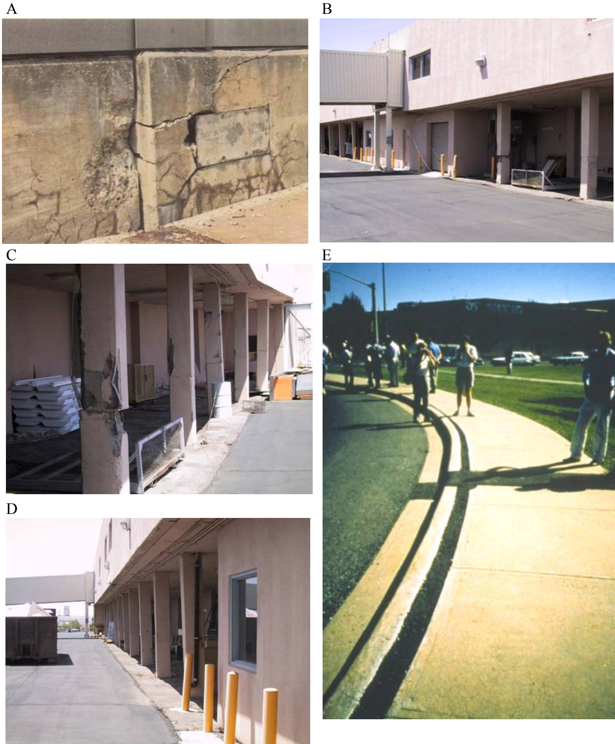
Figure 3.4. A. Relative movement of abutting sections of parapet wall in a bridge structure affected by ASR (Stark 1991). B-D. Expansion of concrete pavement due to ASR (overlaid with asphalt), which pushes against the adjacent building foundation causing shearing of concrete columns. E. Concrete sidewalk made with alkali-carbonate reactive limestone aggregate. Originally, the sidewalk and the curb were adjacent to each other; however, the expansion of the sidewalk created a gap that had to be filled with asphalt.
