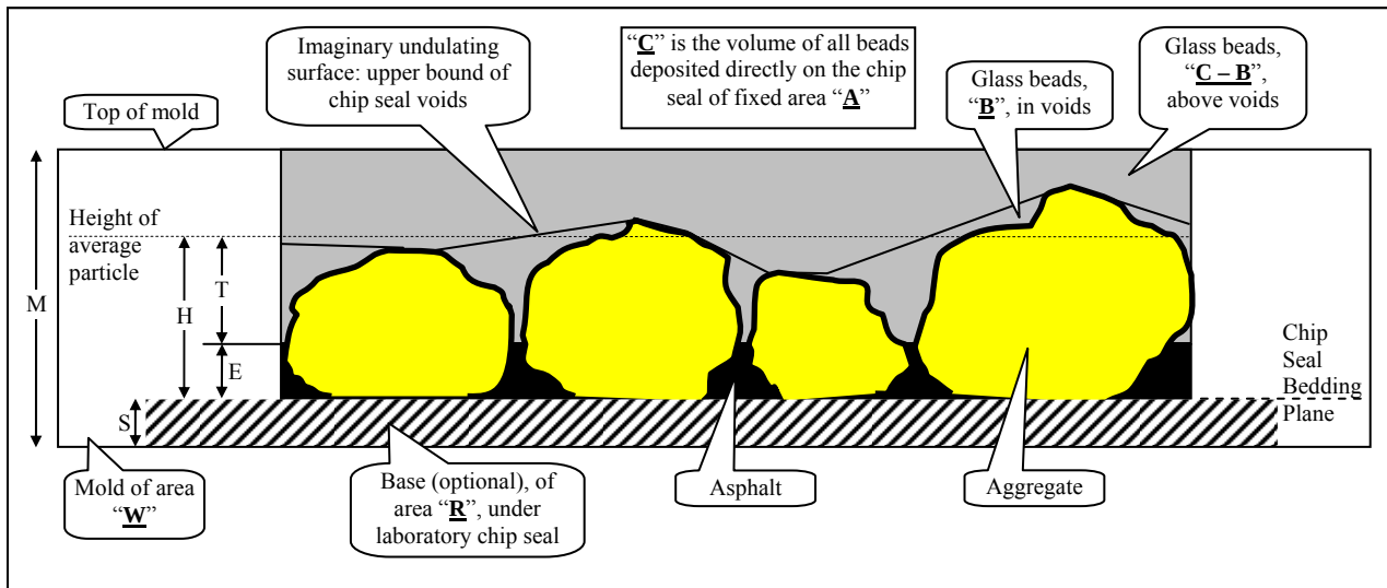
Figure 4—Submerging Procedure
